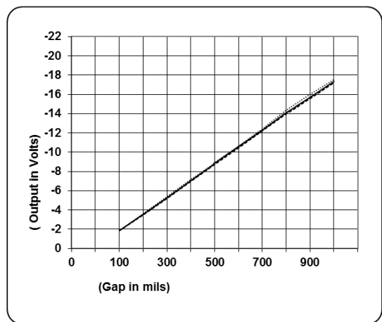
Typical 5m system performance — 25 °C ..... 150 °C - - - 0 °C
